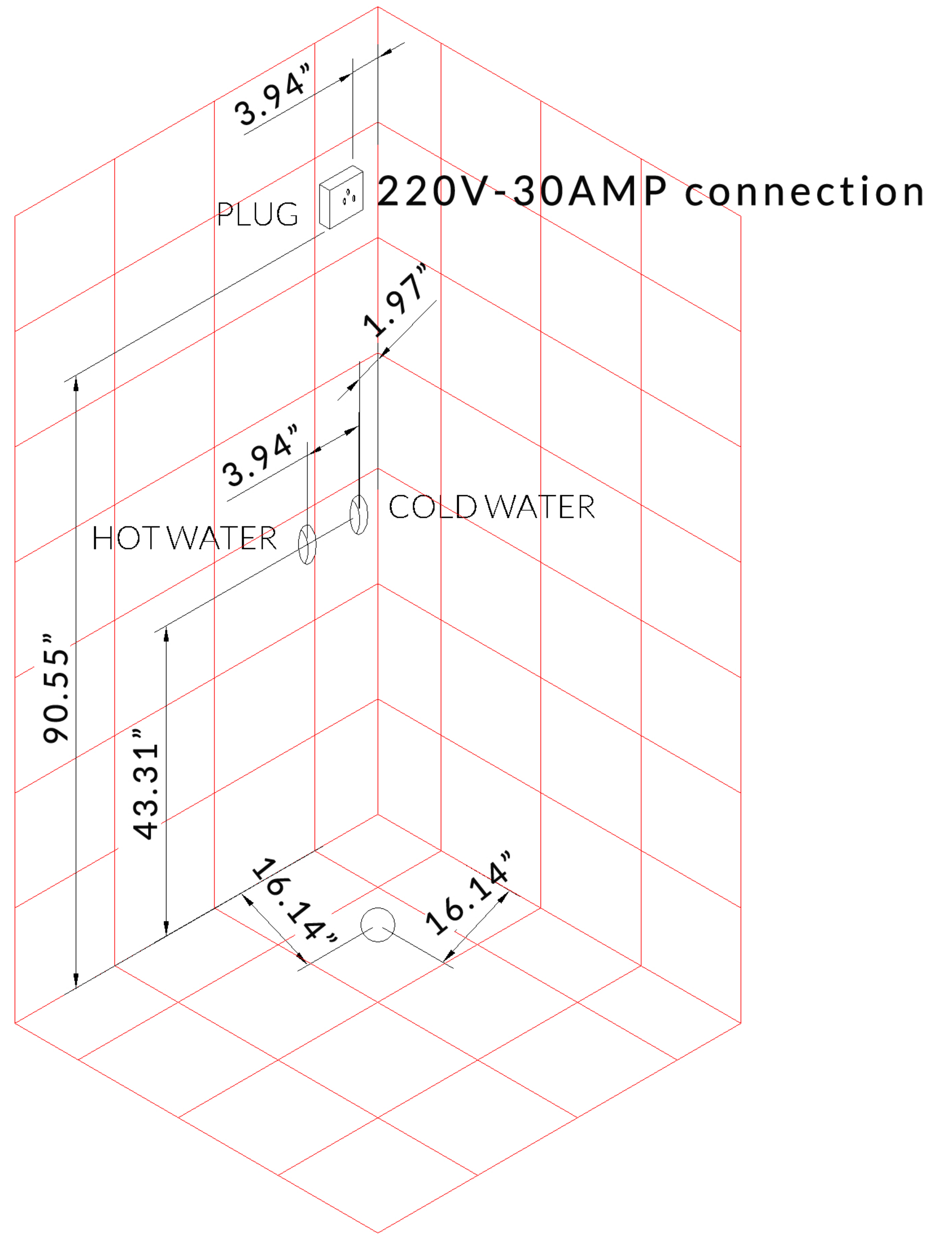
DZ959F8 INSTALLATION(LEFT) DIMENSIONS: 47" x 35" x 89"
