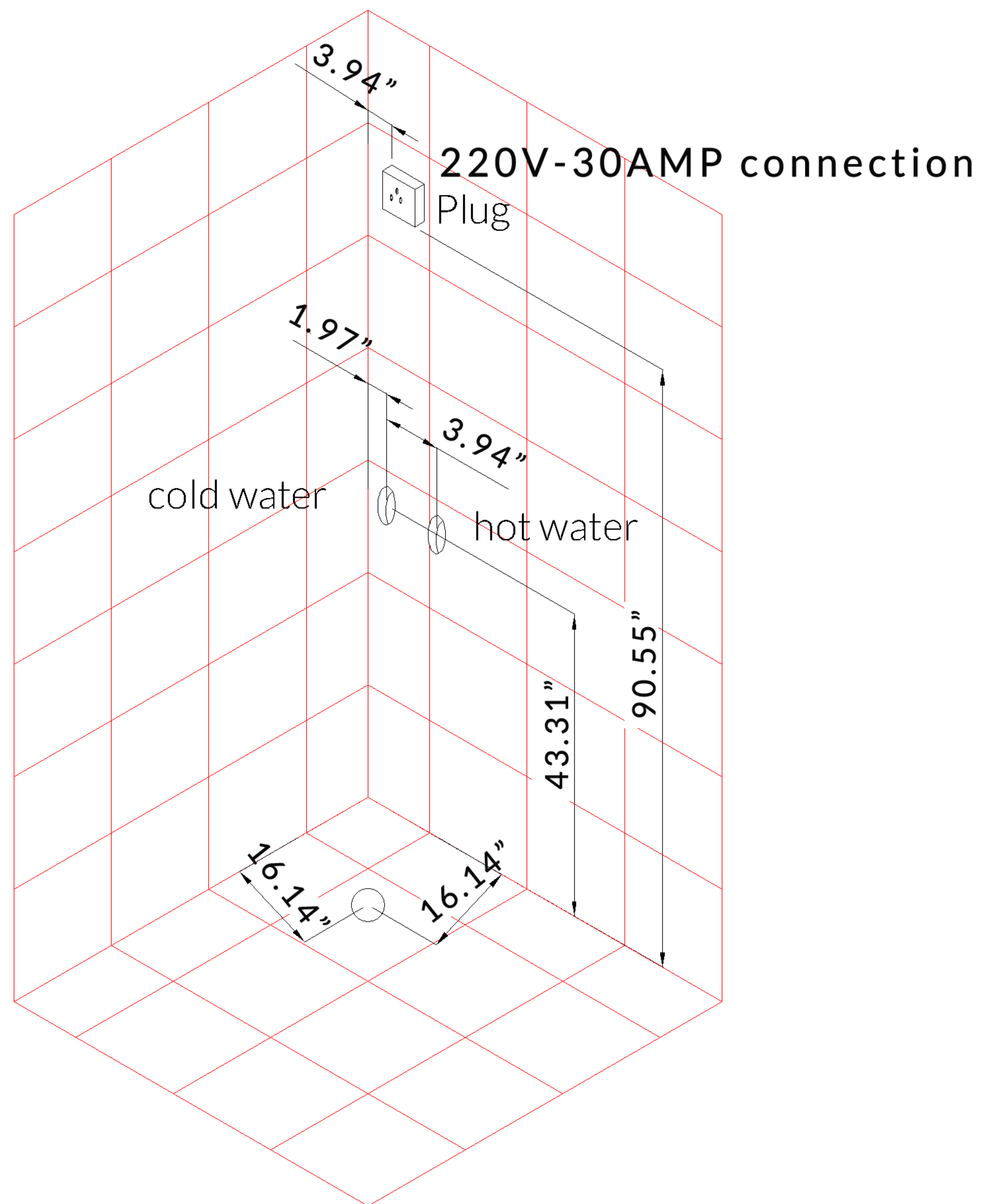
DZ961-1F8 INSTALLATION (RIGHT) DIMENSIONS: 59" x 35" x 89"
